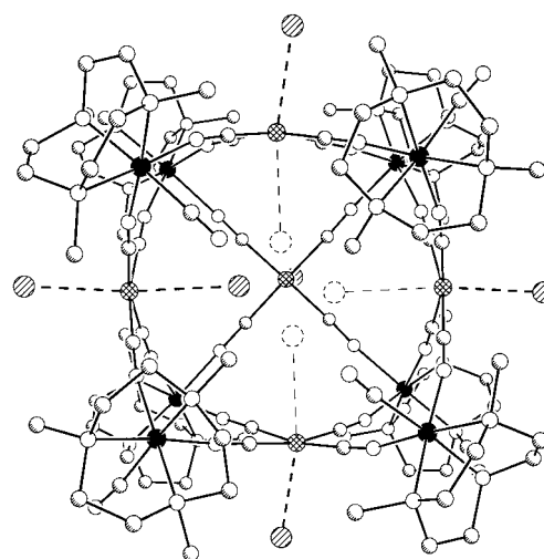
Figure 1. Structure of the [(\text{Me}_3\text{tacn})_8\text{Cr}_8\text{Ni}_5(\text{CN})_{24}]^{10+} cluster and associated \text{I}^- anions, as observed in 1 . Black, cross-hatched, shaded, white, and hatched spheres represent Cr, Ni, C, N and I atoms, respectively; H atoms are omitted for clarity. The cluster has maximal point group symmetry C_{2v} . Selected mean interatomic distances [Å] and angles [°]: Cr–N CN 2.05(6), Cr–C 2.04(5), Ni–C 1.86(2), C–N CN 1.14(3), Ni...I outer 2.91(3), Ni...I inner 3.09(3); N CN –Cr–N CN 87(2), N CN –Cr–C 93(3), Cr–N–C CN 170(4), Cr–C–N 172(4), C–Ni–C 89(1), Ni–C–N 177(1).
